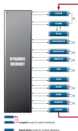
Modules in ASTEC
