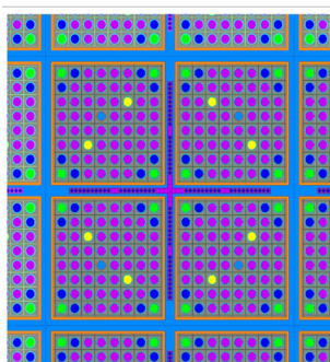
BWR Pin Power Distribution
