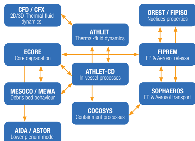
The components of ATHLET-CD code system
