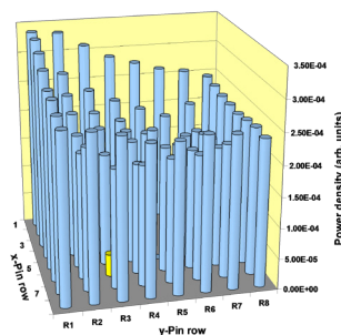
BWR Pin Power Distribution
