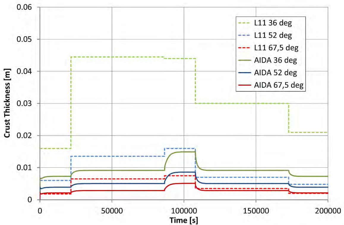
Fig. 5.93 Crust thickness evolution along the wall in L11 test and in AIDA (3.4) simulation at different positions
