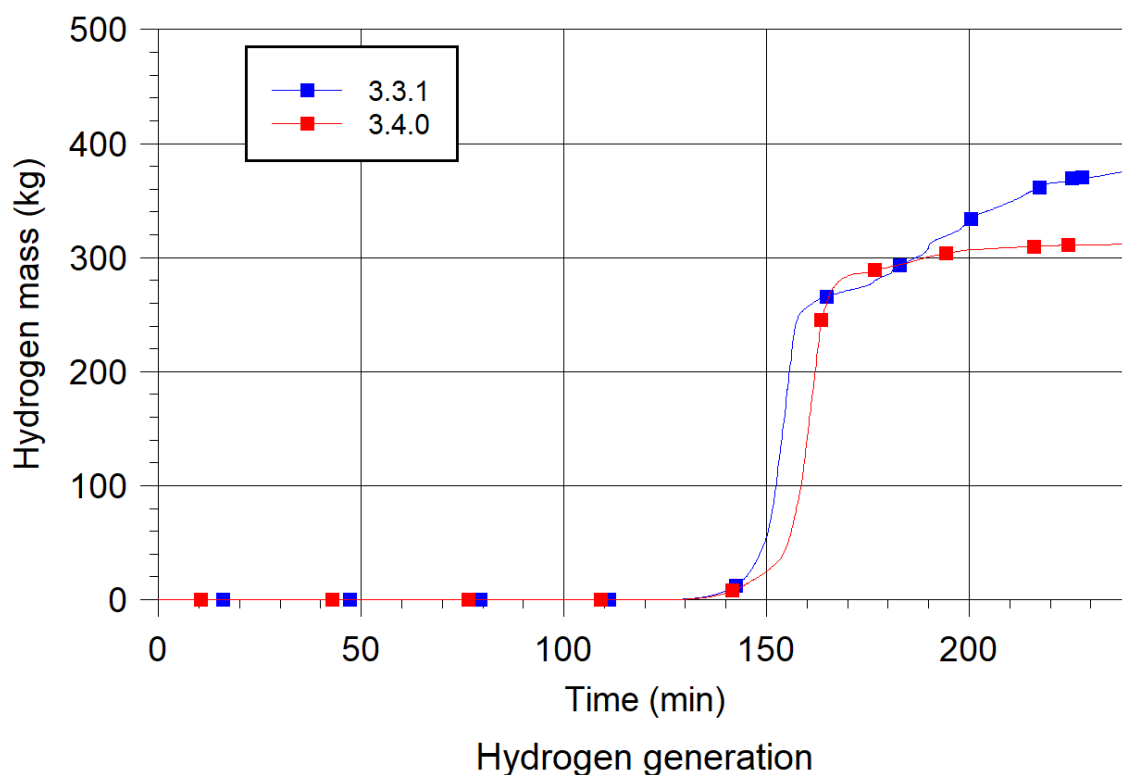
Fig. 5.104 Hydrogen generation calculated with ATHLET-CD 3.3.1 and 3.4.0
