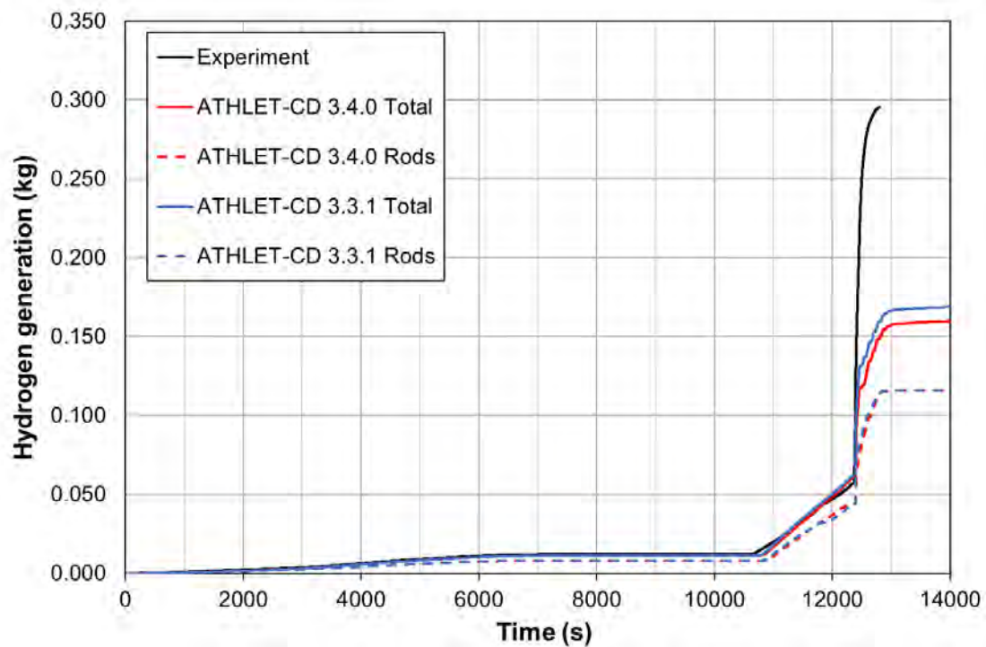
Fig. 5.75 Accumulated mass of generated hydrogen during the test
