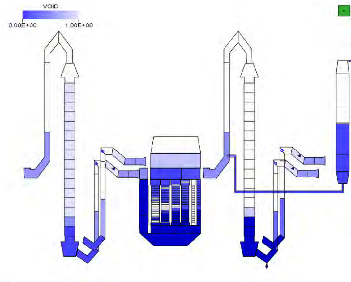
Fig. 5.116 TMI-2 - Plant status at time 210 min – Void fraction in the primary circuit
