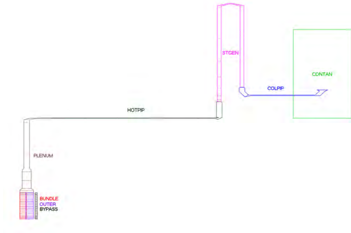
Fig. 5.44 ATHLET-CD model of the FPT-3 test
