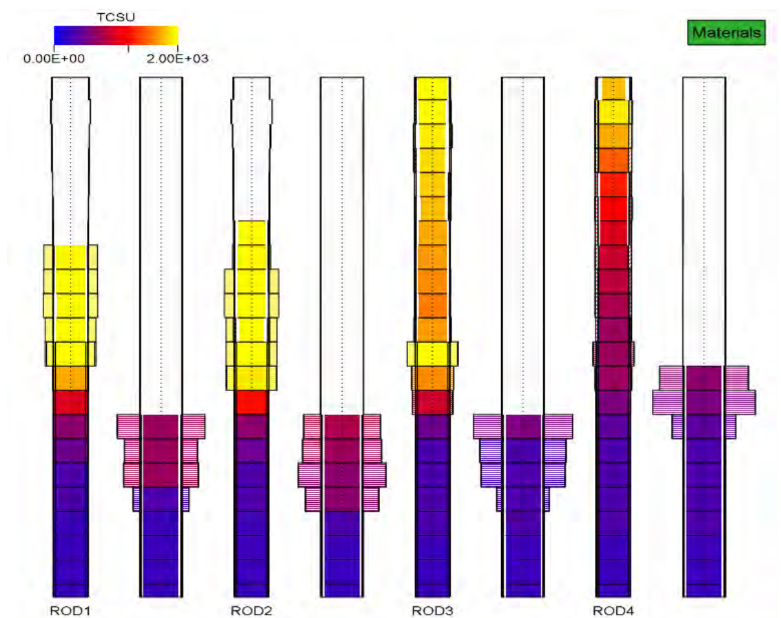
Fig. 5.115 TMI-2 - Plant status at time 174 min – Material distribution and cladding temperatures in the core
