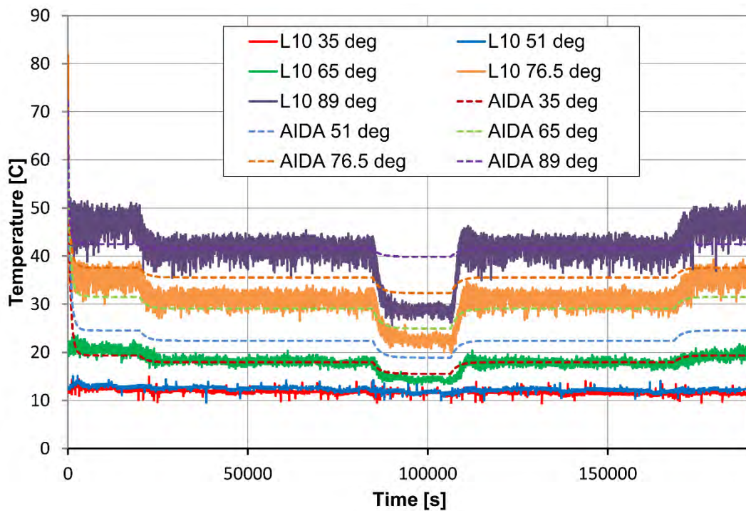
Fig. 5.88 Outer wall temperature evolution at different positions in L10 test and in AIDA (3.4) simulation
