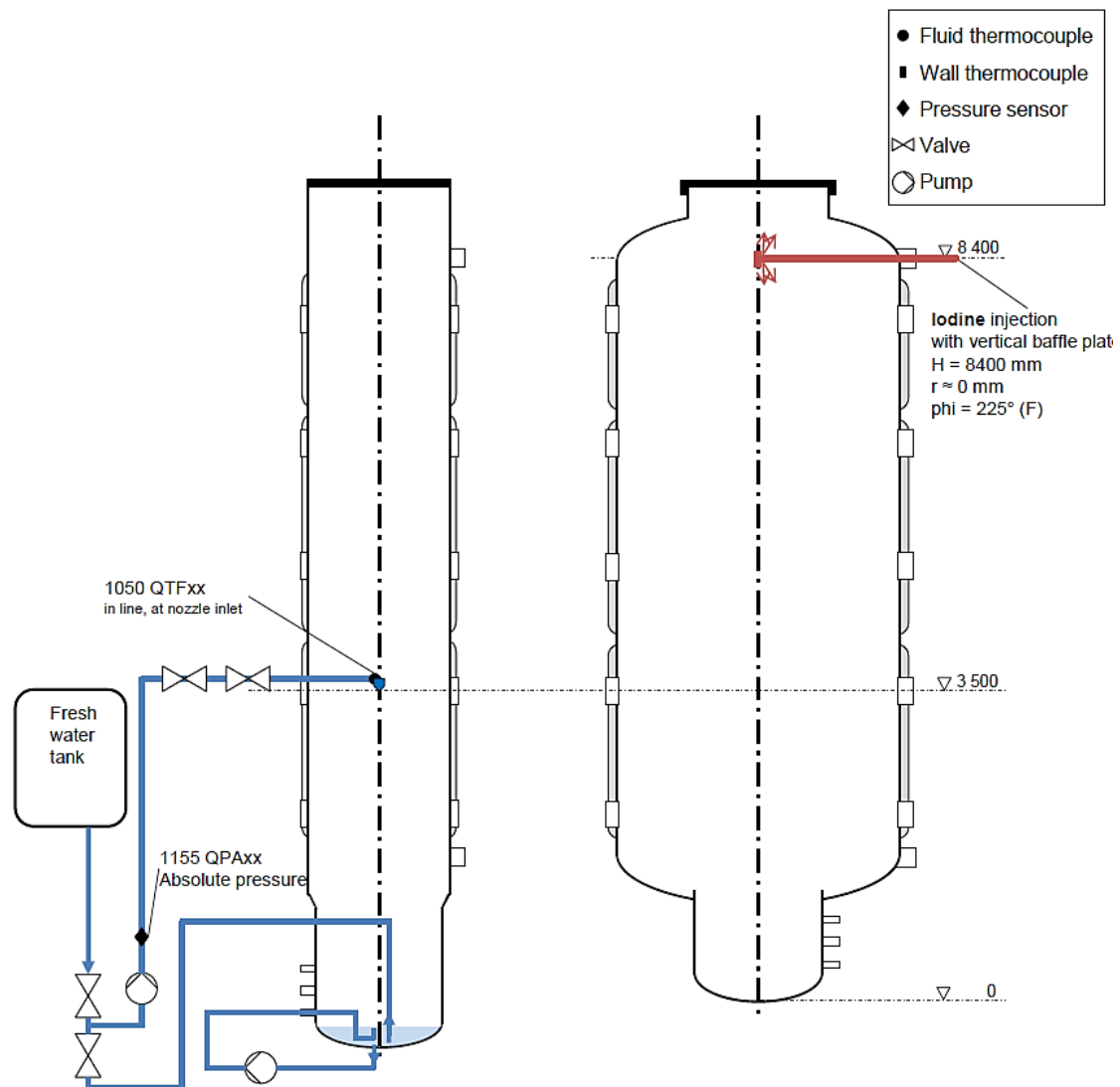
Abb. 2.17 Konfiguration des Tests THAI Iod-31 /FUN 16/
