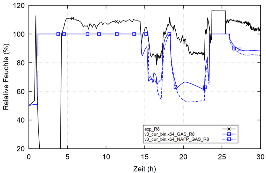
Abb. 2.60 BMC VANAM-M3, relative Feuchte in R8
