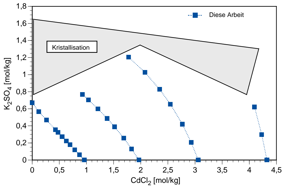
Abb. 2.23 Isopiestic concentrations in the system \text{CdCl}_2 - \text{K}_2\text{SO}_4 - \text{H}_2\text{O}
