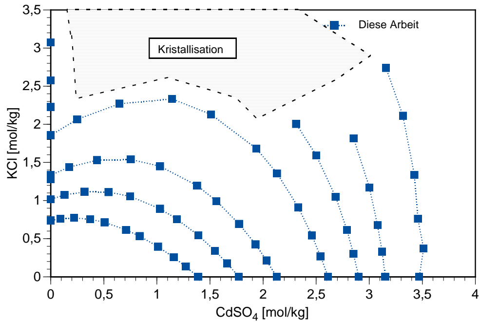
Abb. 2.22 Isopiestic concentrations in the system \text{CdSO}_4 - \text{KCl} - \text{H}_2\text{O}
