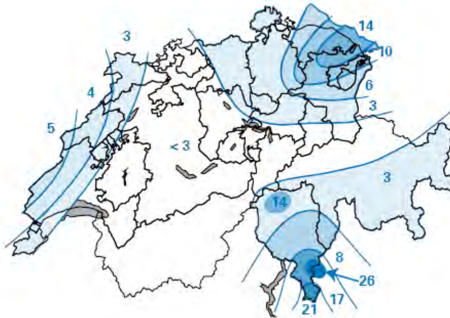
Figure 4-13: Initial distribution pattern of radio-caesium in 1986 after the ChNPP accident (Cs-137 in kBq /m²) /BAG 06a/
