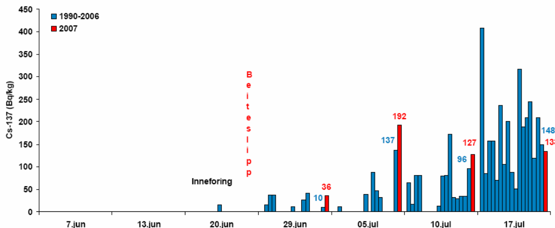
Figure 4-10: Cs 137-concentration in goats milk from Oyster region by means of the caesium binding feed additive Berlin blue
