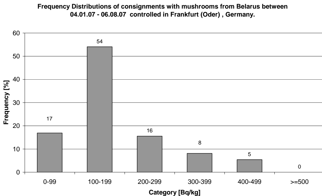
Figure 4-3: Frequency distribution of radio-caesium content in mushrooms from Belarus (148 samples, total of 1236.5 tons)
