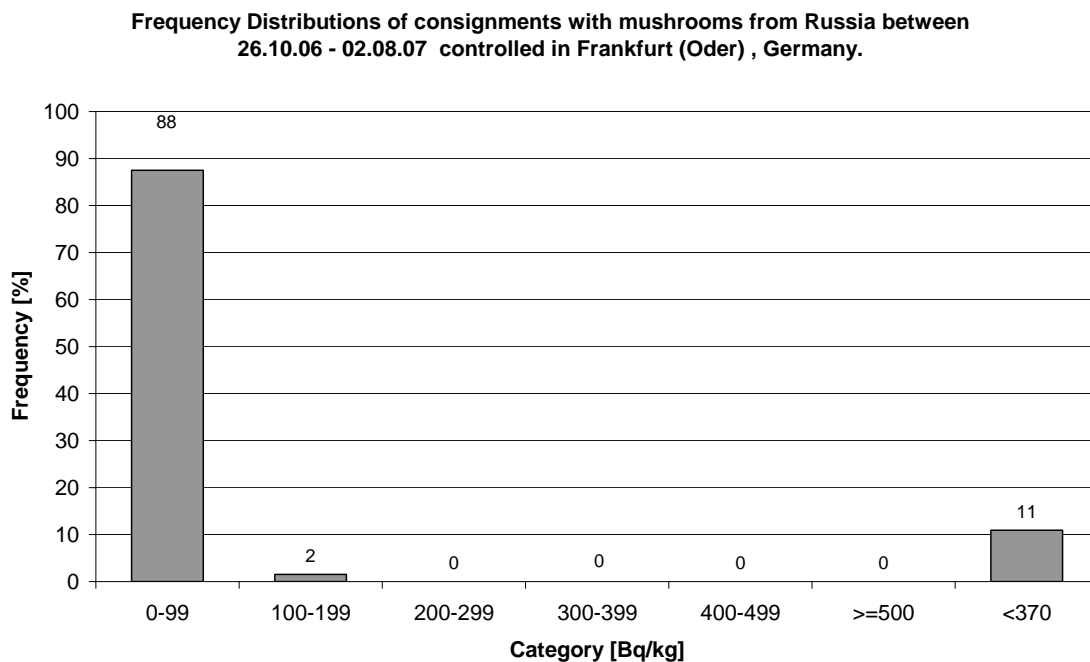
Figure 4-12: Frequency distribution of radio-caesium content in mushrooms from Russia (64 samples, total of 500.6 tons)
